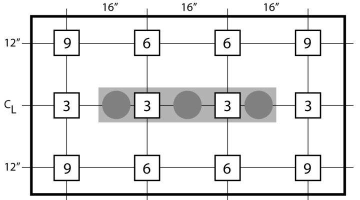
Discharge time in seconds (1000-100V), fan speed set to high; Guardian CR2000 blower 18" from CPM measuring plate; CPM test plate 6" from table; discharge times slightly longer for 230 VAC, 50 Hz unit.
